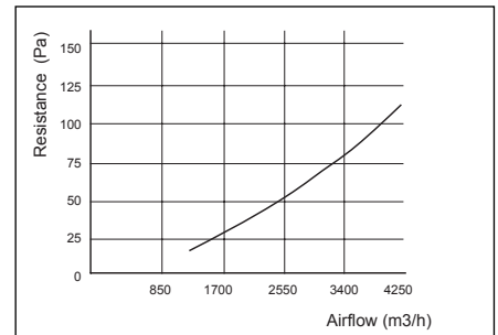
Airflow resistance for a clean 24x24 pad, rated airflow is 3400 m3/h.
